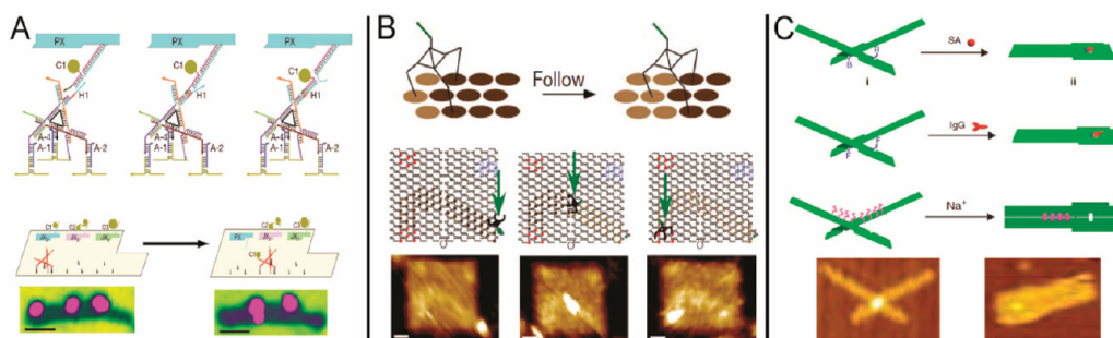
FIGURE 7. Responsive DNA nanodevices: (A) a cargo transportation system consisting of an assembly template, cargo loading apparatus, and DNA walker, 69 (B) walker movement along a 2D deoxyribonucleotide substrate surface, 70 and (C) forceps for sensing various noncovalent interactions. 74 Reproduced with permission from refs 69, 70, and 74. Copyright 2010 and 2011 Nature Publishing Group.
