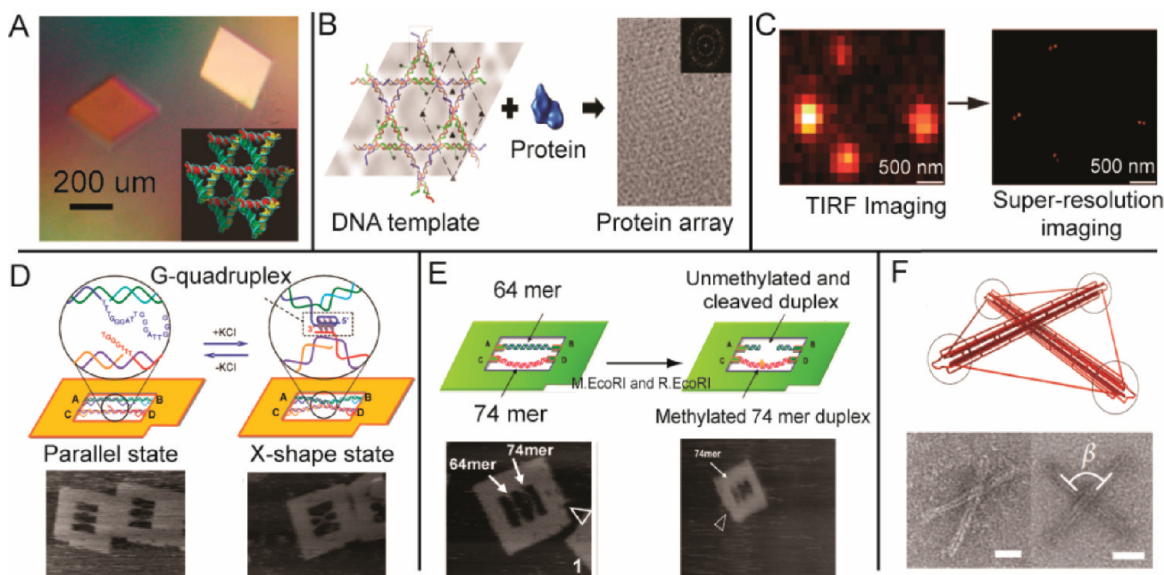
FIGURE 4. DNA nanostructures as biophysical study tools: (A) X-ray diffraction (reproduced with permission from ref 47, copyright 2009 Nature Publishing Group), (B) cyro-EM (reproduced with permission from ref 48, copyright 2011 American Chemical Society), and (C) super-resolution imaging (reproduced with permission from ref 51, copyright 2009 Wiley). Conformational studies of (D) G-quadruplex formation (reproduced with permission from ref 52, copyright 2010 American Chemical Society), (E) DNA methylation (reproduced with permission from ref 53, copyright 2010 American Chemical Society), and (F) constrained intermolecular forces (reproduced with permission from ref 55, copyright 2010 Nature Publishing Group).
